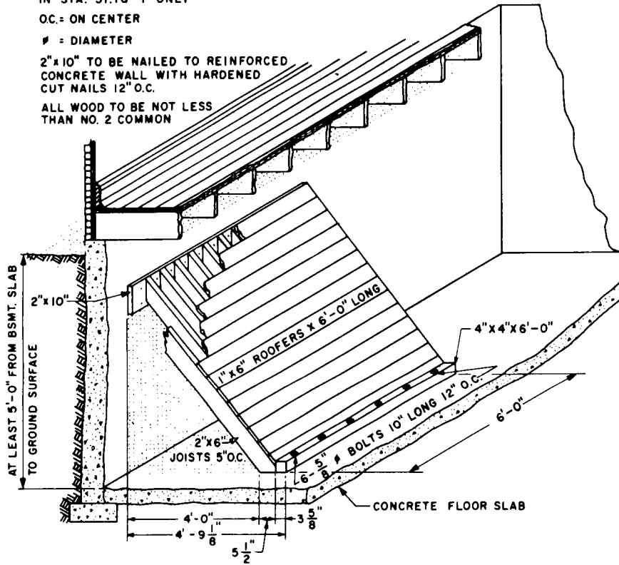
Fig. 3—Sketch of basement lean-to shelter.
